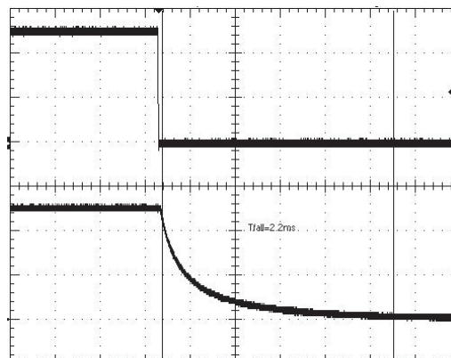
Turn-Off Output Discharge ( V_{IN} = V_{EN} = 5V , V_{OUT} = 5V , C_{OUT} = 4.7\mu F , T_A = 25^\circ C )
