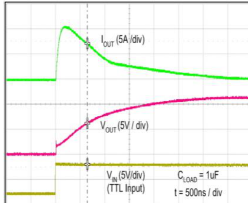
Figure 41. Quasi-Static Source Current with V_{DD} = 12\text{ V} (Note 13)
