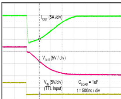
Figure 42. Quasi-Static Sink Current with V_{DD} = 12\text{ V} (Note 13)
