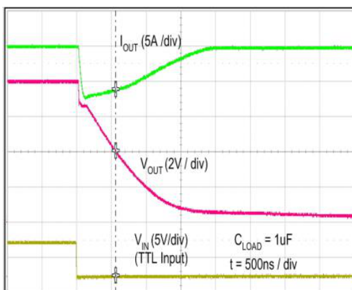
Figure 44. Quasi-Static Sink Current with V_{DD} = 8\text{ V} (Note 13)
