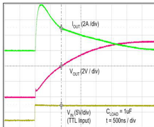
Figure 43. Quasi-Static Source Current with V_{DD} = 8\text{ V} (Note 13)
