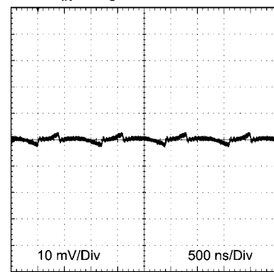
输出波纹 12V_{IN} 3.3V_O @ 5A, BW = 20 MHz
