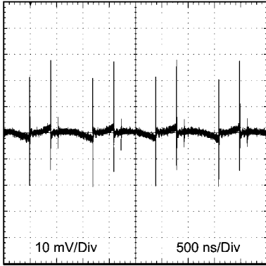
输出波纹 12V_{IN} 3.3V_O @ 5A BW = 250\text{ MHz}
