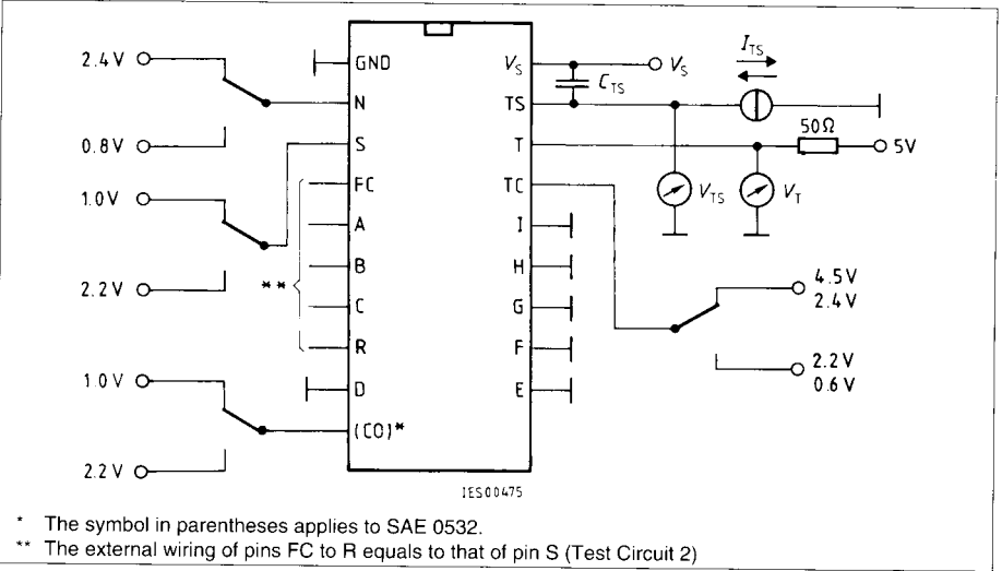
Test Circuit 2
