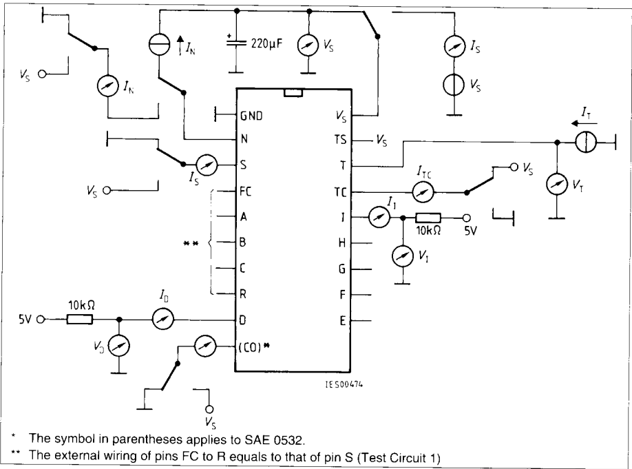
Test Circuit 1
