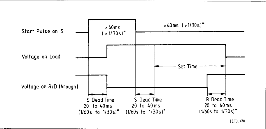
Figure 2 Dropout Delay
