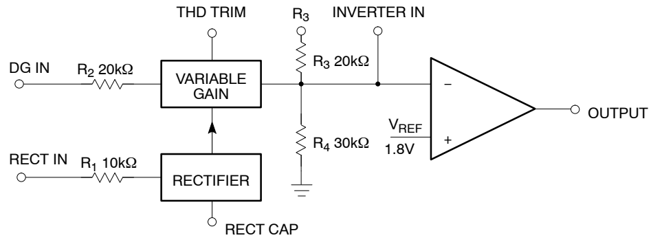
Figure 1. Block Diagram
