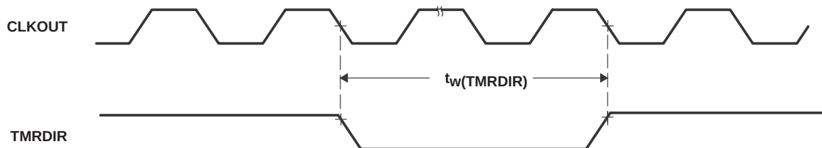
Figure 26. Capture/TMRDIR Timing
