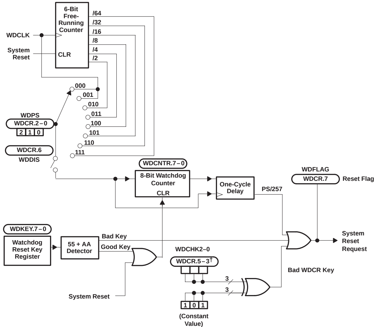
Figure 12. Block Diagram of the WD Module
