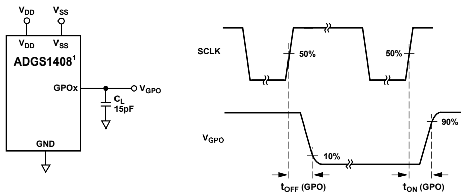
Figure 43. GPOx Timing, t ON (GPO) and t OFF (GPO)
