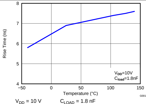
Figure 13. Rise Time vs Temperature
