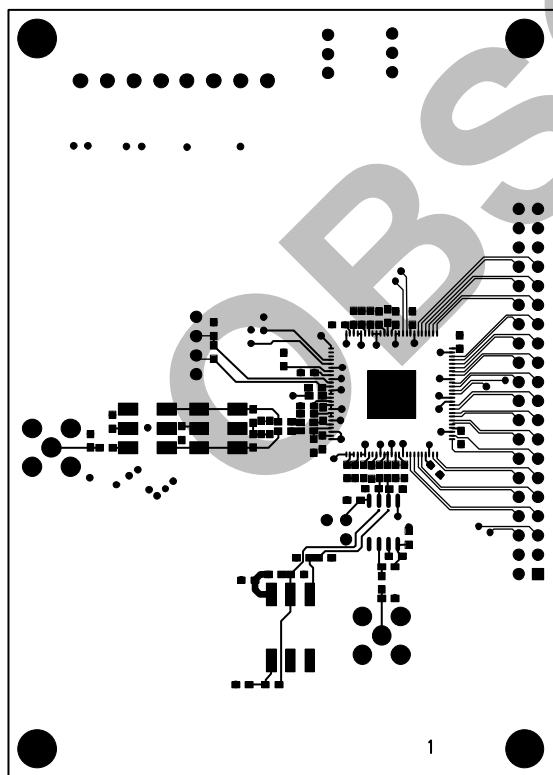
Figure 49. PCB Top Side Copper Routing
