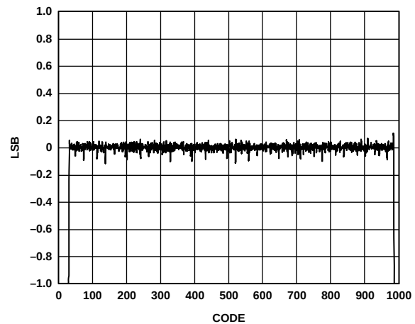
Figure 32. Typical DNL Plot ( A_{IN} = 10.3 \text{ MHz} @ -0.5 \text{ dBFS} ) 170/200 MSPS
