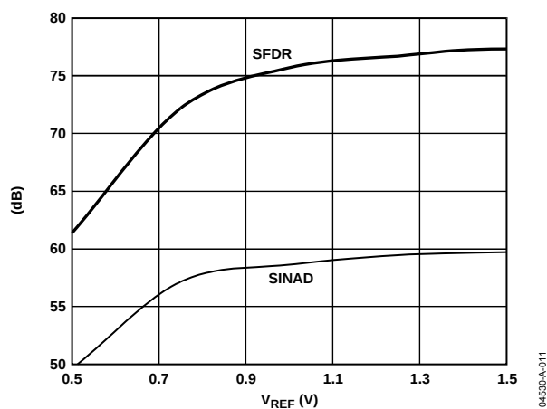
Figure 26. Sinad, SFDR vs. VREF in External Reference Mode (AIN = 70 MHz @ -0.5 dBFS, 200 MSPS)
