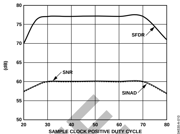
Figure 24. SINAD and SFDR vs. Clock Pulse Width High (AIN = 10.3 MHz @ -0.5 dBFS, 200 MSPS)
