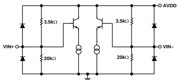
Figure 5. Analog Inputs
