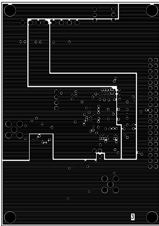
Figure 51. PCB Split Power Plane
