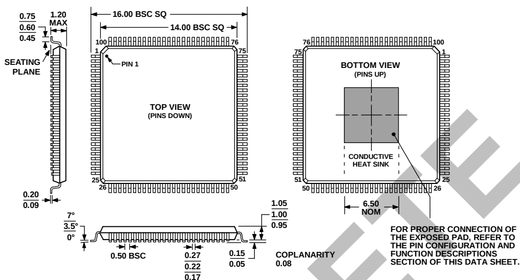
Figure 54. 100-Lead Thin Quad Flat Package, Exposed Pad [TQFP_EP] (SV-100)
