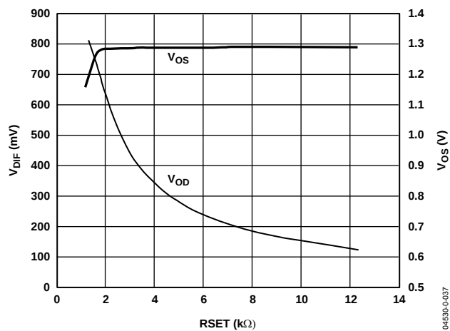
Figure 38. LVDS Output Swing, Common-Mode Voltage vs. R_{SET} , Placed at LVDSBIAS (Both Speed Grades)
