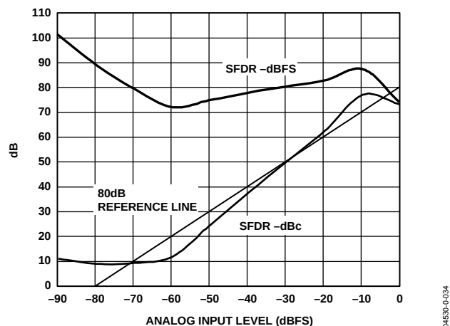
Figure 33. SFDR vs. AIN Input Level 10.3 MHz, AIN @ 170 MSPS
