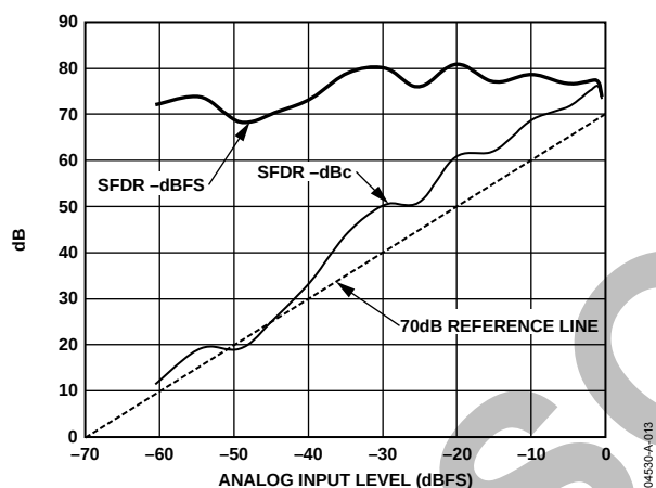
Figure 34. SFDR vs. AIN Input Level 70 MHz, AIN @ 200 MSPS
