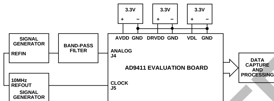
Figure 44. Evaluation Board Connections
