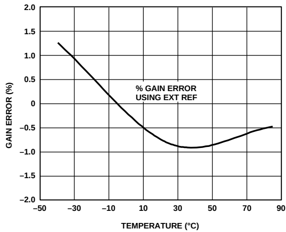
Figure 27. Full-Scale Gain Error vs. Temperature ( A_{IN} = 10.3 \text{ MHz} @ -0.5 \text{ dBFS} , 170/200 MSPS)
