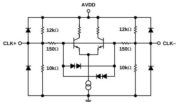
Figure 4. Clock Inputs
