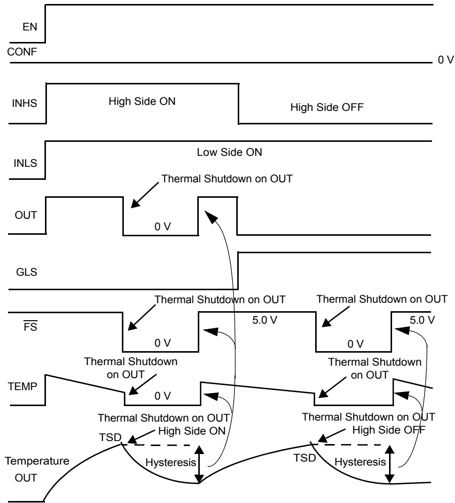
Figure 3. Overtemperature on Output
