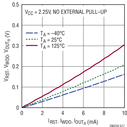
\overline{\text{RST}} , \overline{\text{WDO}} , \text{OUT}_n V_{OL} vs Pull-Down Current
