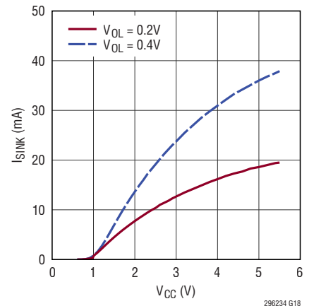
Output Logic Low, I_{SINK} vs V_{CC} \overline{\text{RST}} , \overline{\text{WDO}} , \text{OUT}_n
