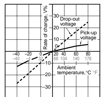
5.-(1) Ambient temperature characteristics (1 Form A)
