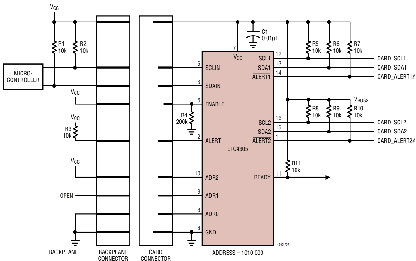
Figure 7. Hot-Swapping Application
