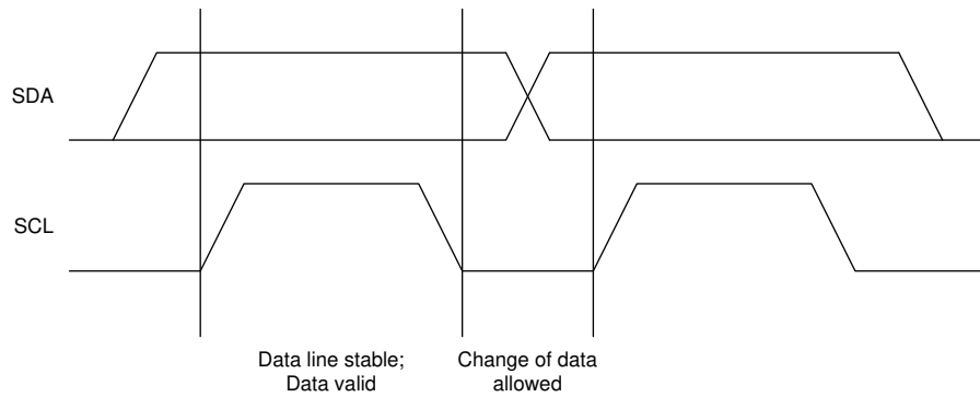
图 9-12. Bit Transfer on the I²C Bus
