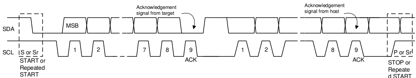
图 9-14. Data Transfer on the I²C Bus
