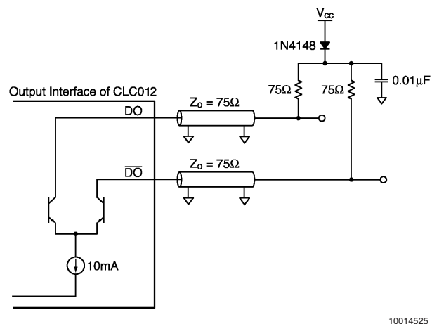
FIGURE 5. Differential Load Terminated Output Interface
