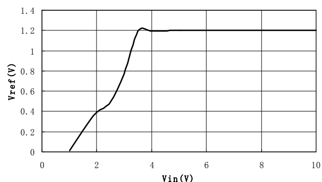
V_{ref} vs. V_{in} at low supply voltage
