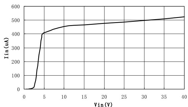
Supply Current vs. V_{in} (Operating)
