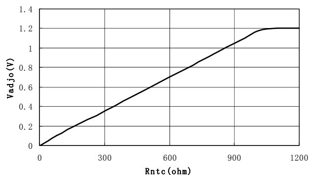
V_{adjo} vs. R_{ntc} R_{ntc} falling, R_{th}=1k\Omega
