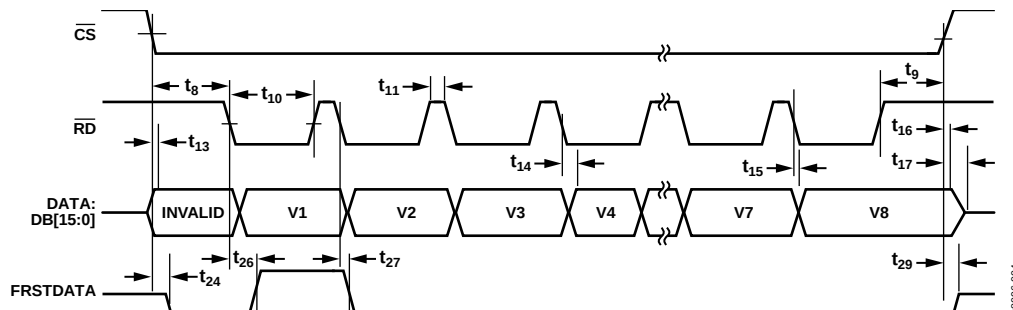
Figure 4. Parallel Mode, Separate \overline{CS} and \overline{RD} Pulses
