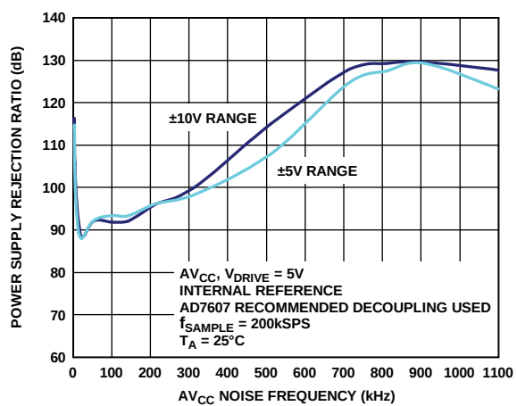
Figure 28. PSRR
