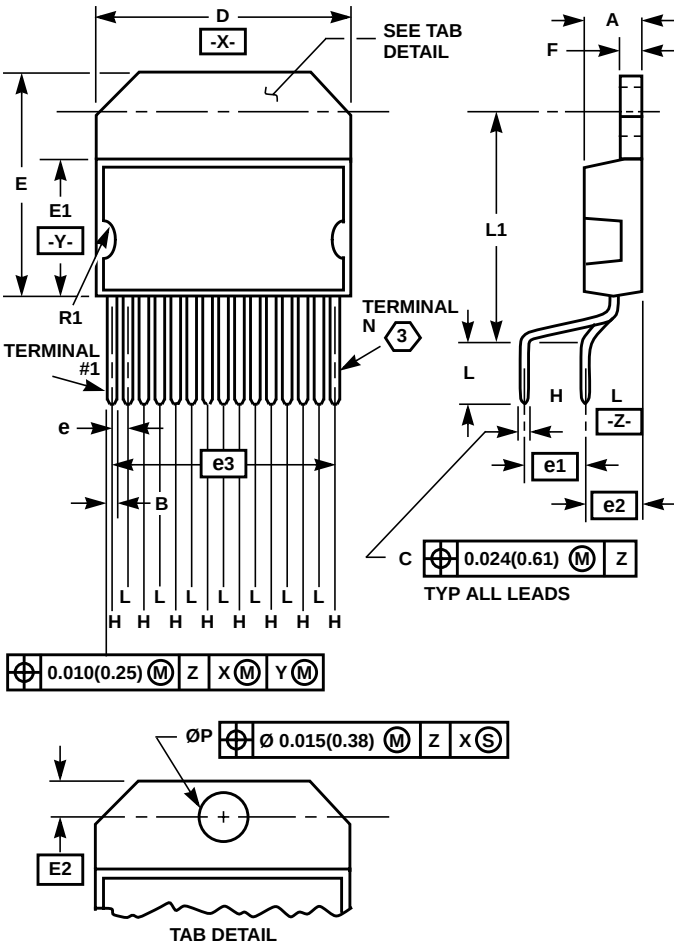
15 LEAD PLASTIC SINGLE-IN-LINE PACKAGE STAGGERED VERTICAL LEAD FORM
