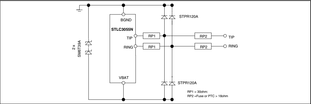
Figure 19. Simplified configuration for indoor overvoltage protection
