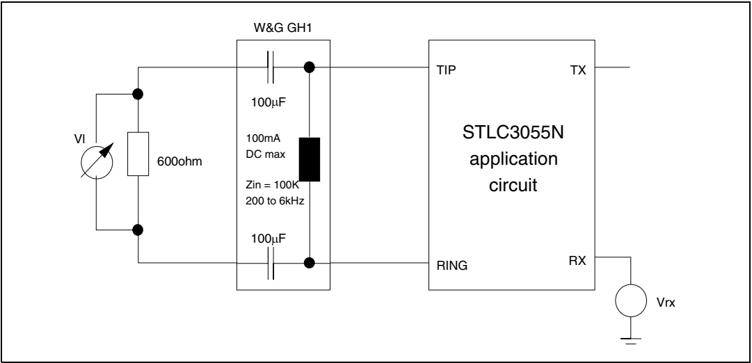
Figure 13. G_{42} receive gain G_{42} = 20\text{Log}|V_I/V_{rx}|
