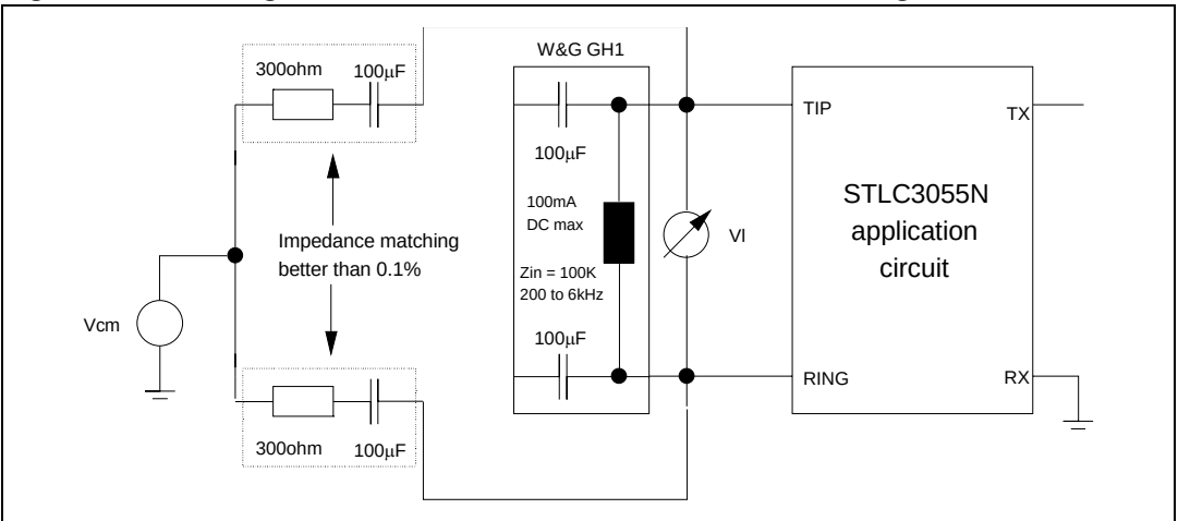
Figure 15. L/T longitudinal to transversal conversion L/T = 20\text{Log}|V_{cm}/V_I|
