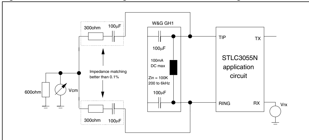
Figure 16. T/L transversal to longitudinal conversion T/L = 20\text{Log}|V_{rx}/V_{cm}|
