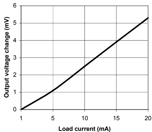
Load regulation
