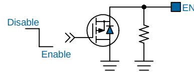
Figure 11. Enable Sequence Control
