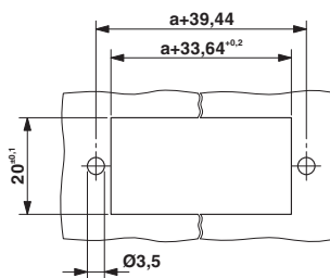
Sheet metal cutout for screw connection.
