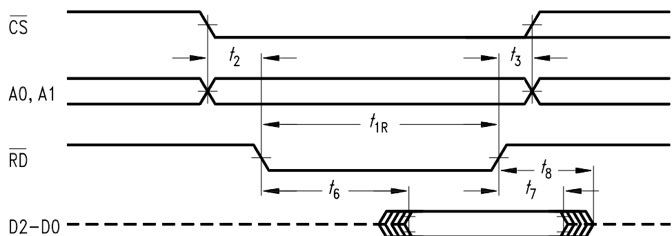
Read Timing
