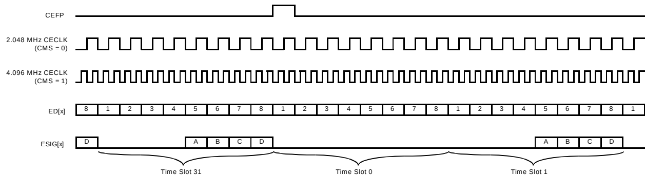
Figure 38 - Non-Multiplexed Transmit Backplane at 2.048/4.096 MHz
