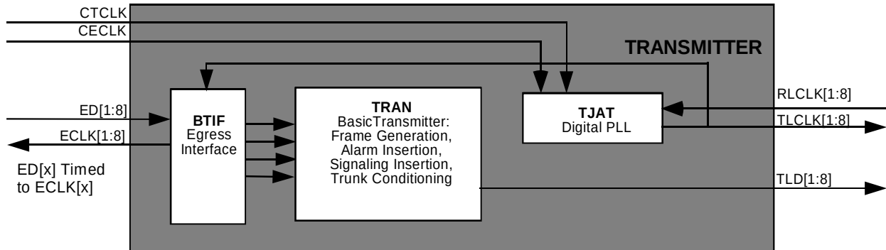
Figure 12 - Clock Master: NxTS.
