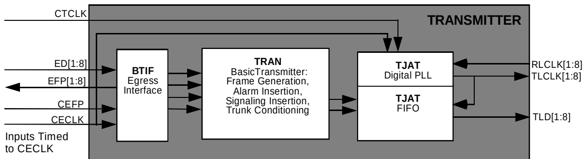
Figure 13 - Clock Slave: EFP Enabled.
