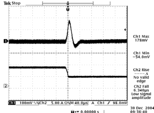
100% to 50% load 12 Vdc Input 1.8 Vdc Output
