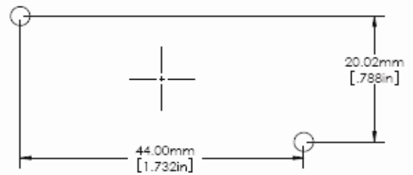
HOLE PATTERN B
