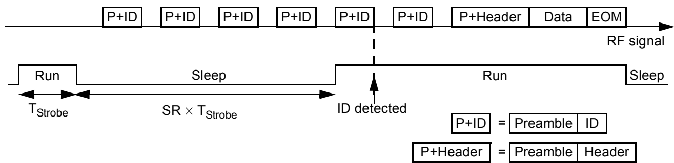
Figure 6: Complete telegram with ID detection
