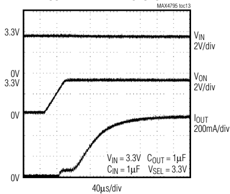
MAX4797/MAX4798 CURRENT-LIMIT RESPONSE
