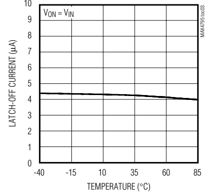
LATCH-OFF CURRENT vs. TEMPERATURE
