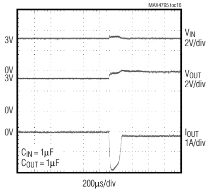
MAX4797/MAX4798 REVERSE CURRENT LIMIT
