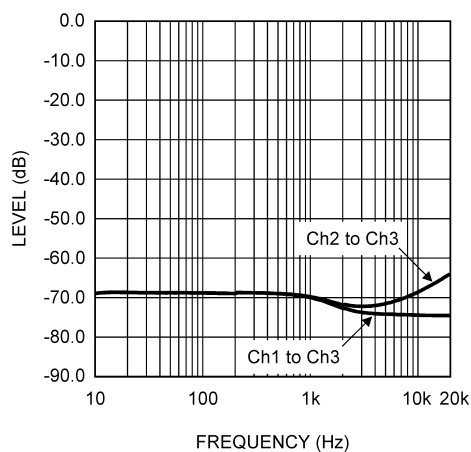
Crosstalk vs Frequency \pm 21\text{V} , P_{\text{OUT}} = 10\text{W} , Channel 3 R_L = 8\Omega , 80kHz BW
