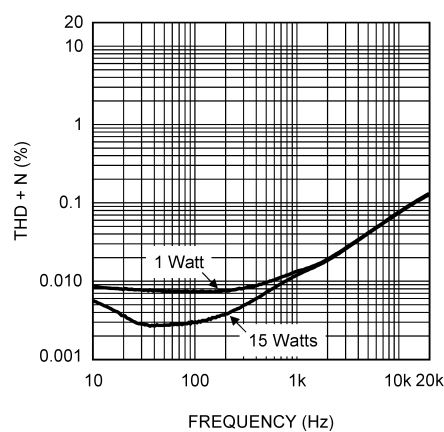
THD+N vs Frequency \pm 17\text{V} , P_{\text{OUT}} = 1\text{W} & 15\text{W} , Chs 1 & 3 in Bridge Mode (Note 15), R_L = 8\Omega , 80kHz BW
