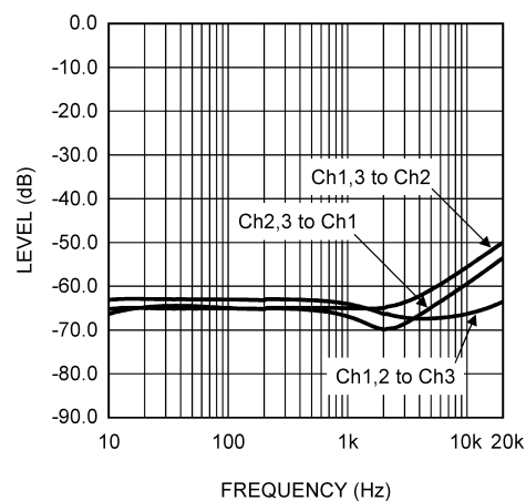
Two Channels On Crosstalk vs Frequency \pm 21\text{V} , P_{\text{OUT}} = 10\text{W} , R_L = 8\Omega , 80kHz BW
