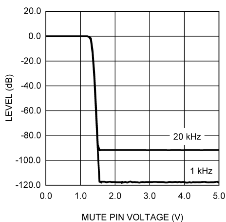
Mute Attenuation vs Mute Pin Voltage P_{\text{OUT}} = 10\text{W/Channel}
