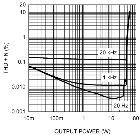
THD+N vs Output Power \pm 17V , Chs 1 & 3 in Bridge Mode (Note 15) R_L = 8\Omega , 80kHz BW
