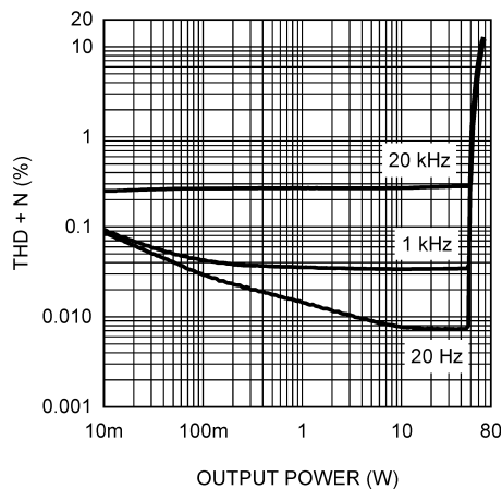
THD+N vs Output Power \pm 19V , All Chs in Parallel Mode (Note 16) R_L = 2\Omega , 80kHz BW
