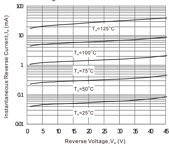
Fig. 3 - Reverse Characteristics
