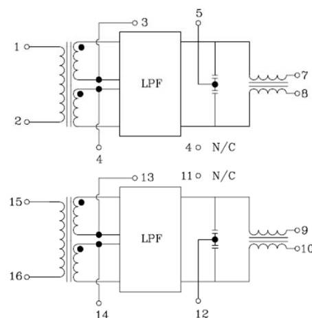
SCHEMATIC
