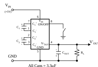
Figure 1. AMS682 Test Circuit
