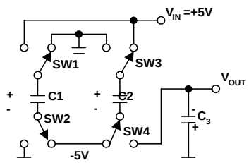
Figure 2. Charge Pump - Phase 1
