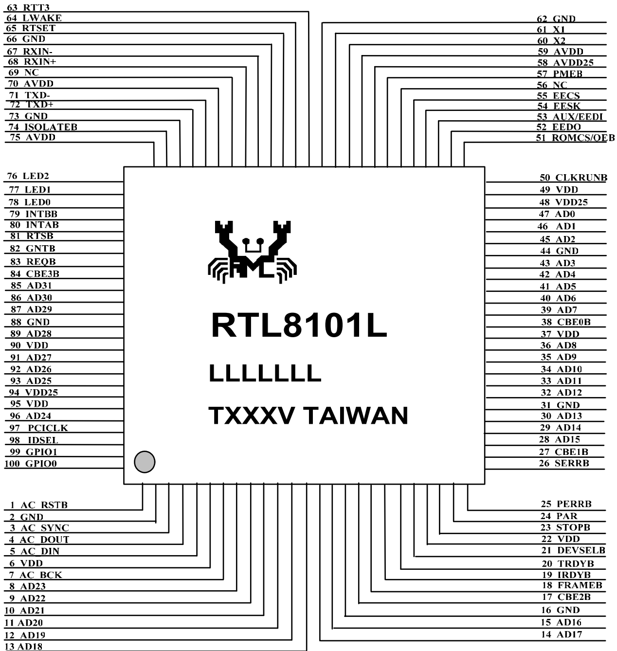
Figure 2. Pin Assignments
