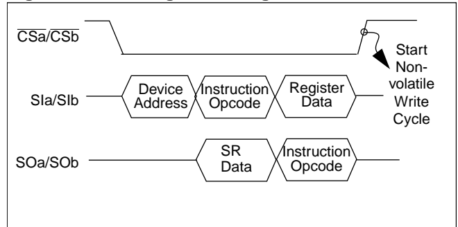
Figure 9. Write Register - Single
