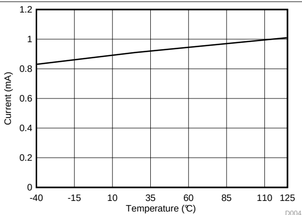
Figure 9. I_{nom} With No Load and 10- \Omega Load
