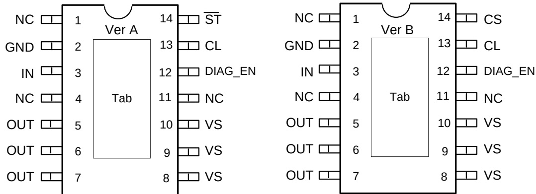
PWP Package 14-Pin HTSSOP Top View
