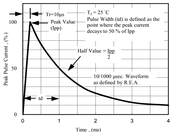
Fig. 5 - Pulse Waveform
