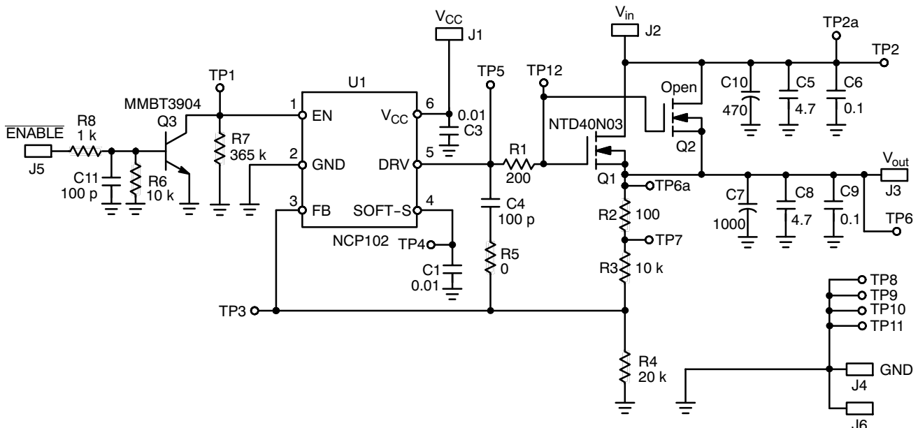
Figure 14. Circuit Schematic
