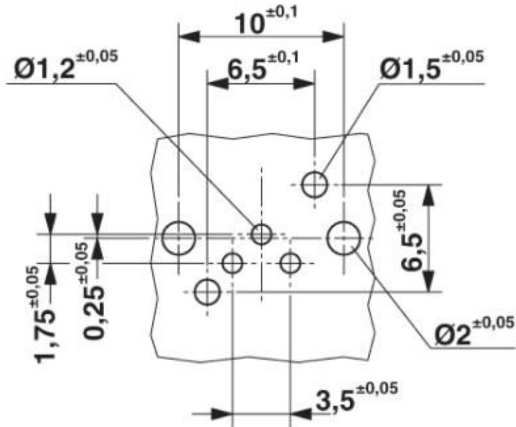
Drilling diagram
