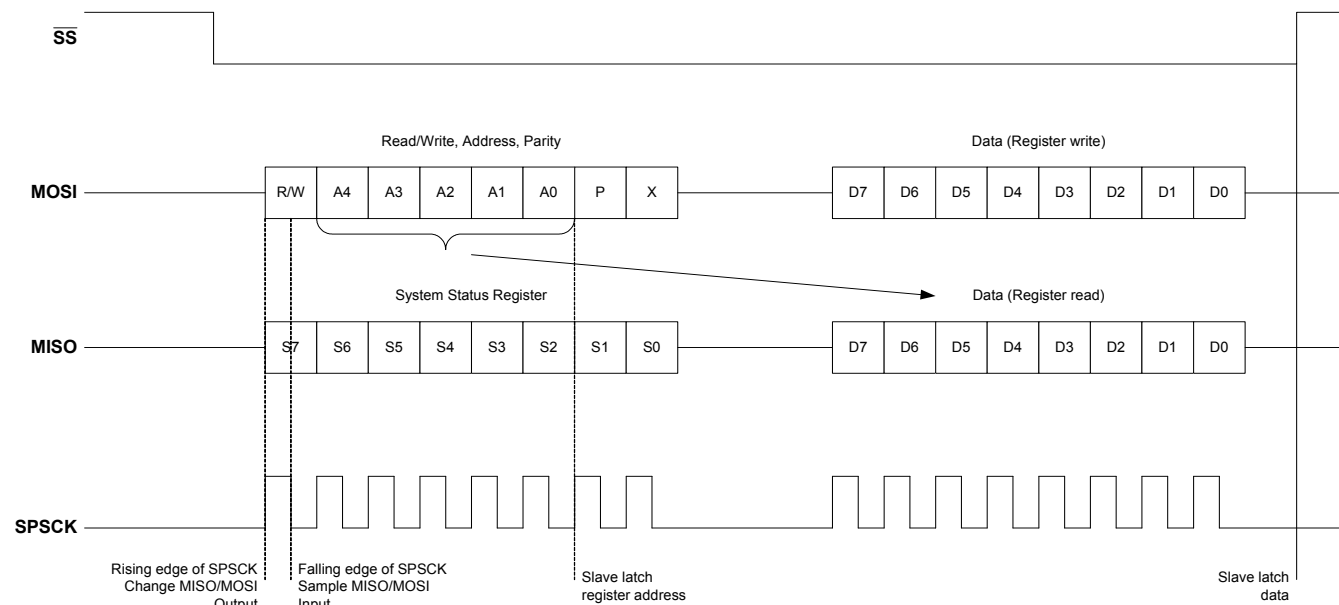
Figure 31. SPI Protocol
