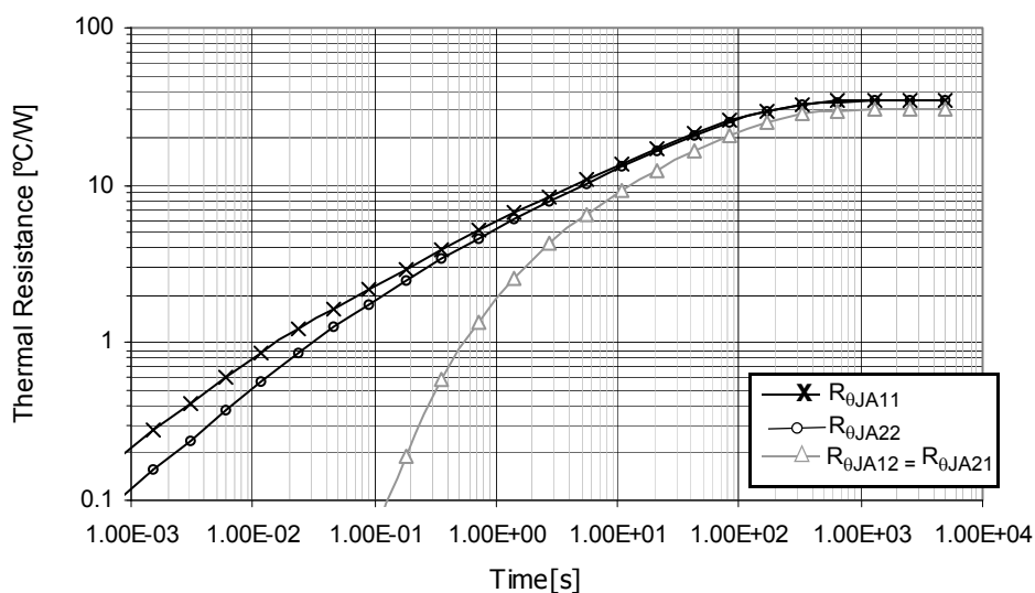
Figure 39. Transient Thermal Resistance R θJA (1.0 W Step Response) Device on Thermal Test Board Area A = 600 (mm²)
