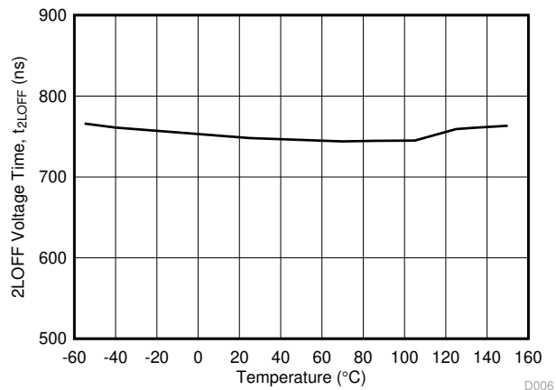
Figure 6-28. t 2LOFF 2-Level Turn Off Time vs. Temperature
