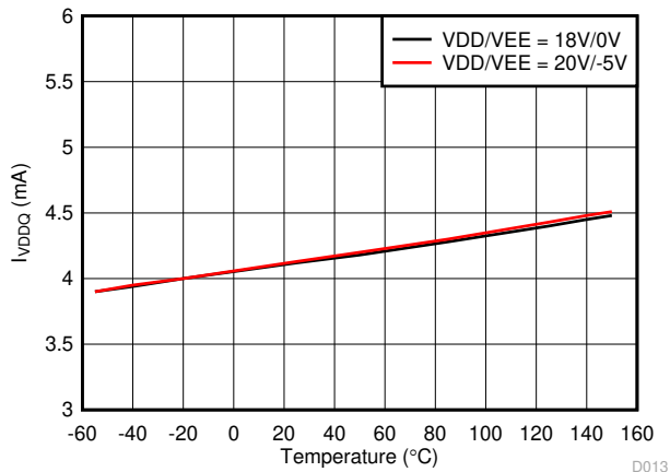
Figure 6-10. I_{VDDQ} Supply Current vs. Temperature
