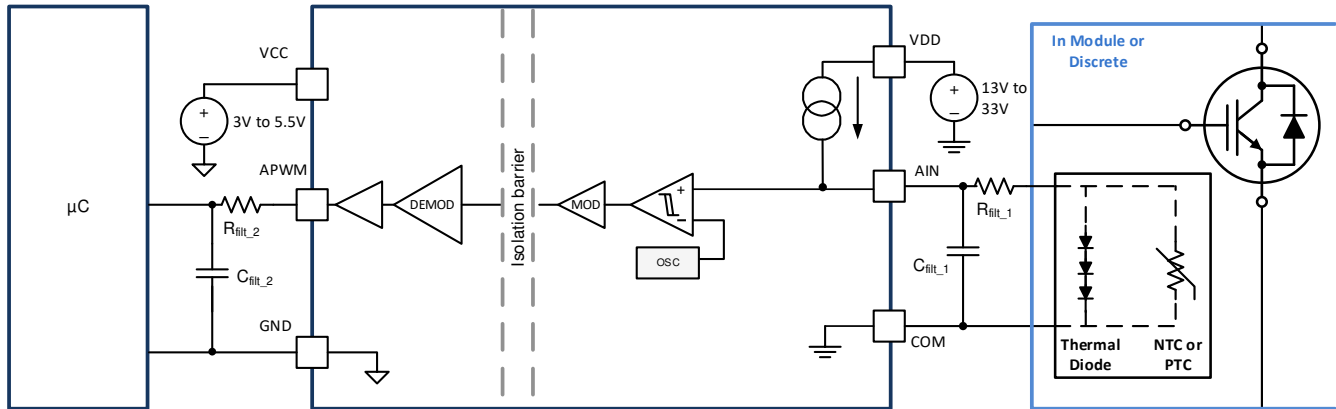
Figure 9-12. APWM Channel with Filtered Output
