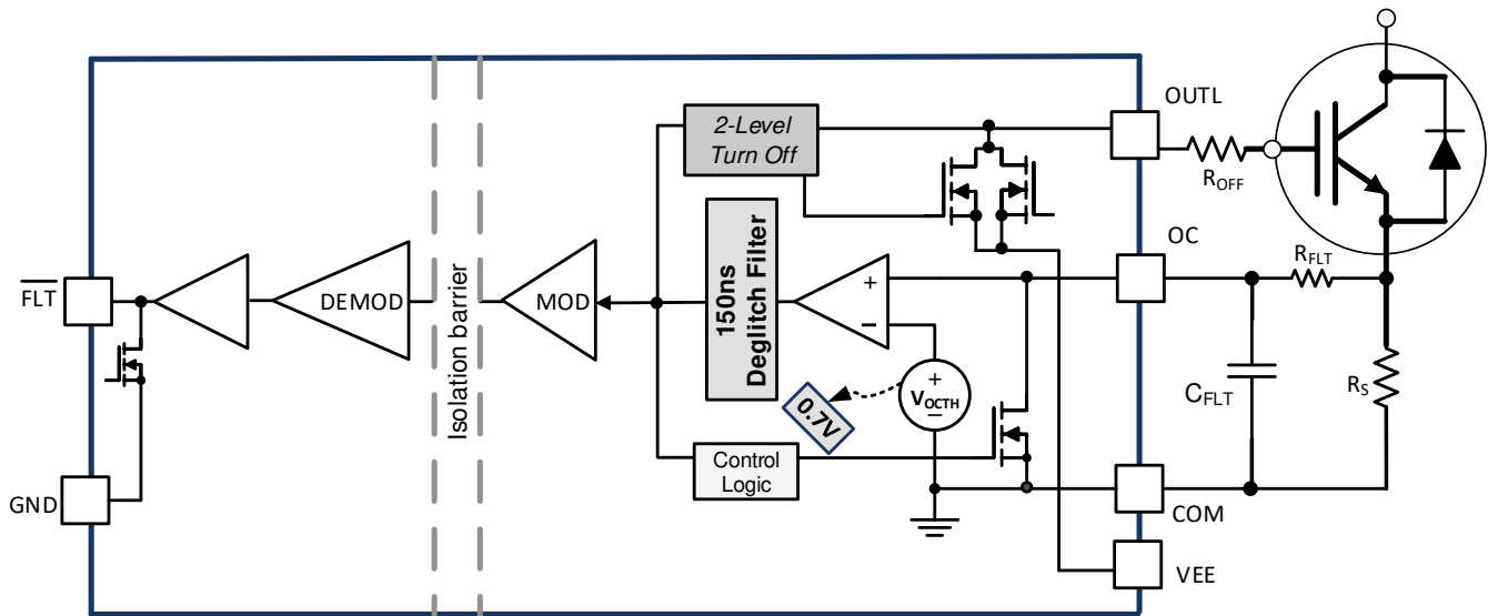
Figure 8-6. 2-Level Turn-off
