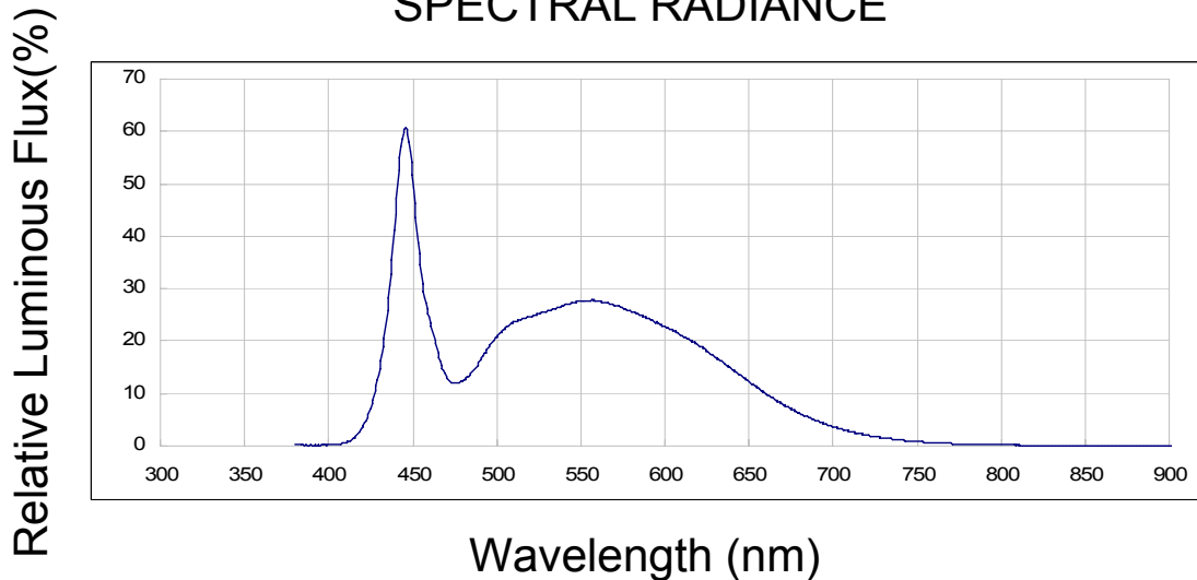
Fig.5 Luminous Spectrum ( T_a=25^\circ\text{C} )
