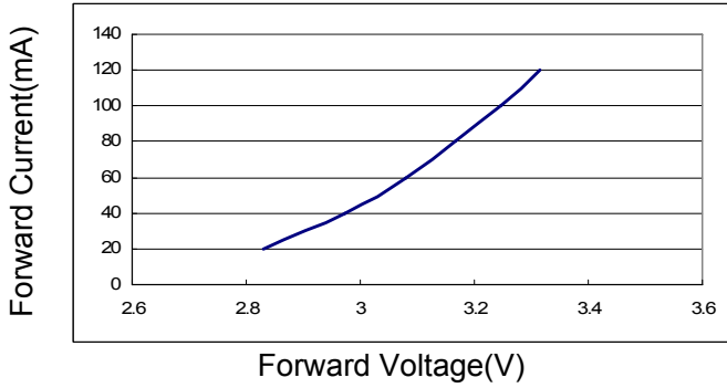
Fig.1 Forward current vs. Forward Voltage
