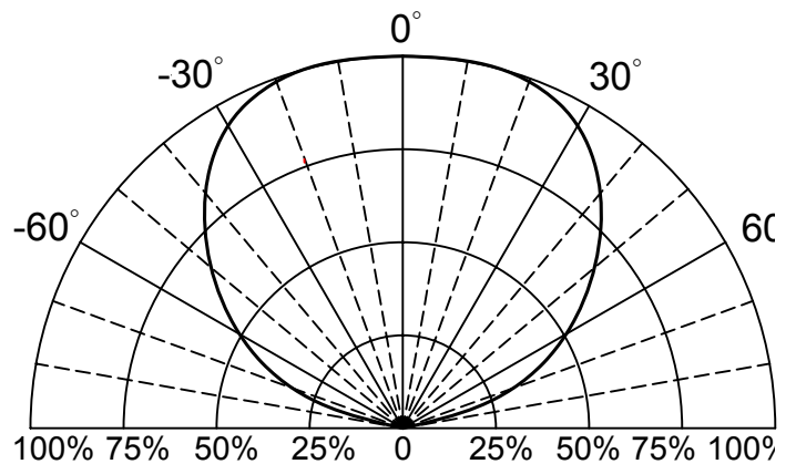
Fig.4 Directivity Radiation
