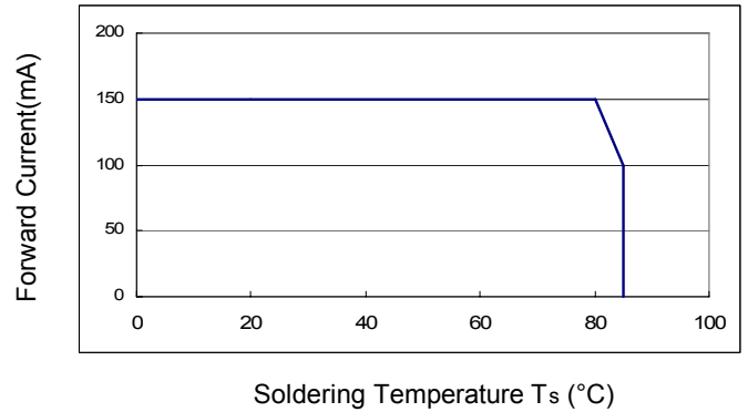
Fig.3 Max. Driving Forward Current VS. Soldering Temperature
