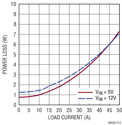
Figure 14. 1.0V OUT Power Loss Curve
