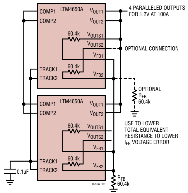
Figure 2. 4-Phase Parallel Configurations
