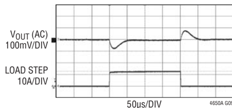
3.3V Dual Phase Single Output Load Transient Response (Ceramic Cap)
