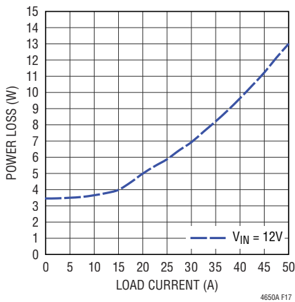
Figure 17. 5V OUT Power Loss Curve
