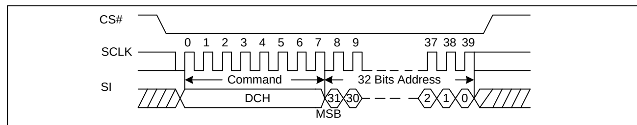
Figure 46 64KB Block Erase with 4-Byte Address Sequence Diagram (ADS=0 or ADS=1)
