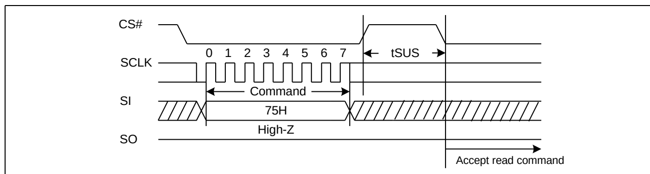
Figure 60 Program/Erase Suspend Sequence Diagram
