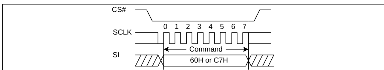
Figure 47 Chip Erase Sequence Diagram
