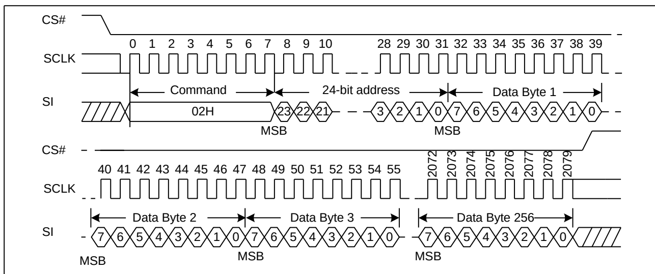
Figure 32 Page Program Sequence Diagram (ADS=0)
