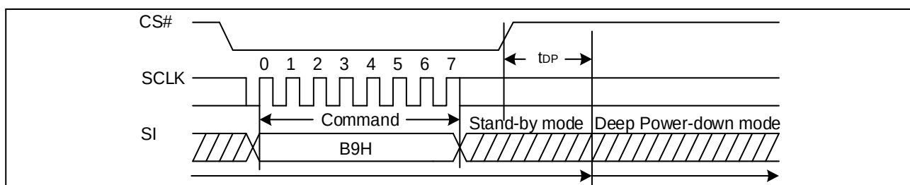
Figure 48 Deep Power-Down Sequence Diagram
