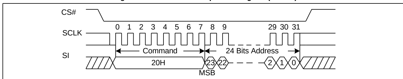
Figure 39 Sector Erase Sequence Diagram (ADS=1)
