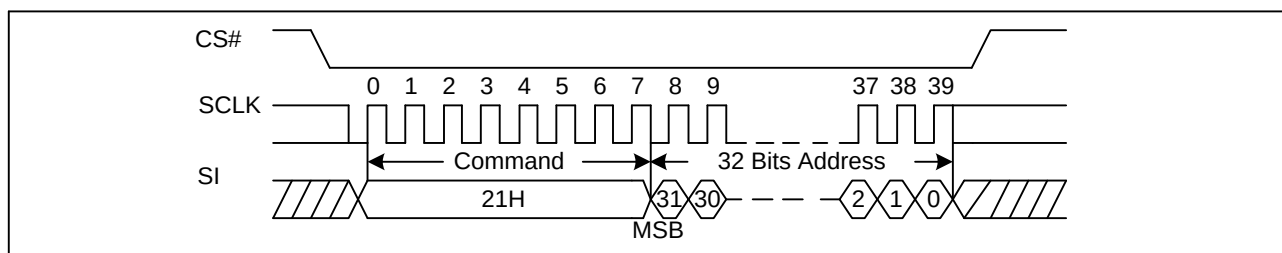
Figure 40 Sector Erase with 4-Byte Address Sequence Diagram (ADS=0 or ADS=1)
