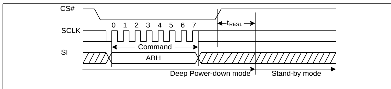
Figure 54 Release Power-Down Sequence Diagram
