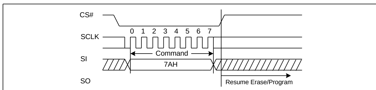
Figure 61 Program/Erase Resume Sequence Diagram
