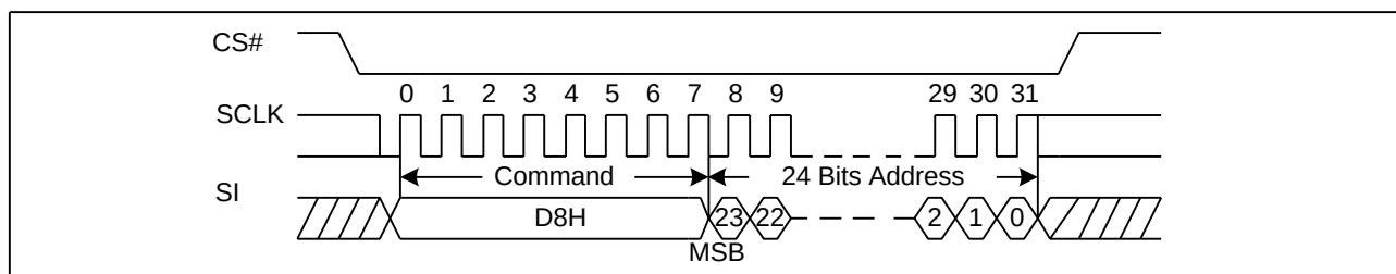
Figure 45 64KB Block Erase Sequence Diagram (ADS=1)
