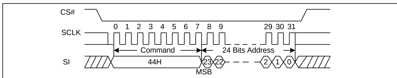
Figure 62 Erase Security Registers command Sequence Diagram (ADS=0)
