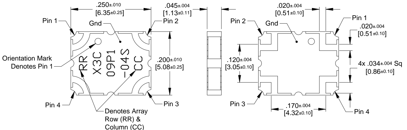
Dimensions are in Inches [Millimeters] X3C09P1-04S Mechanical Outline
