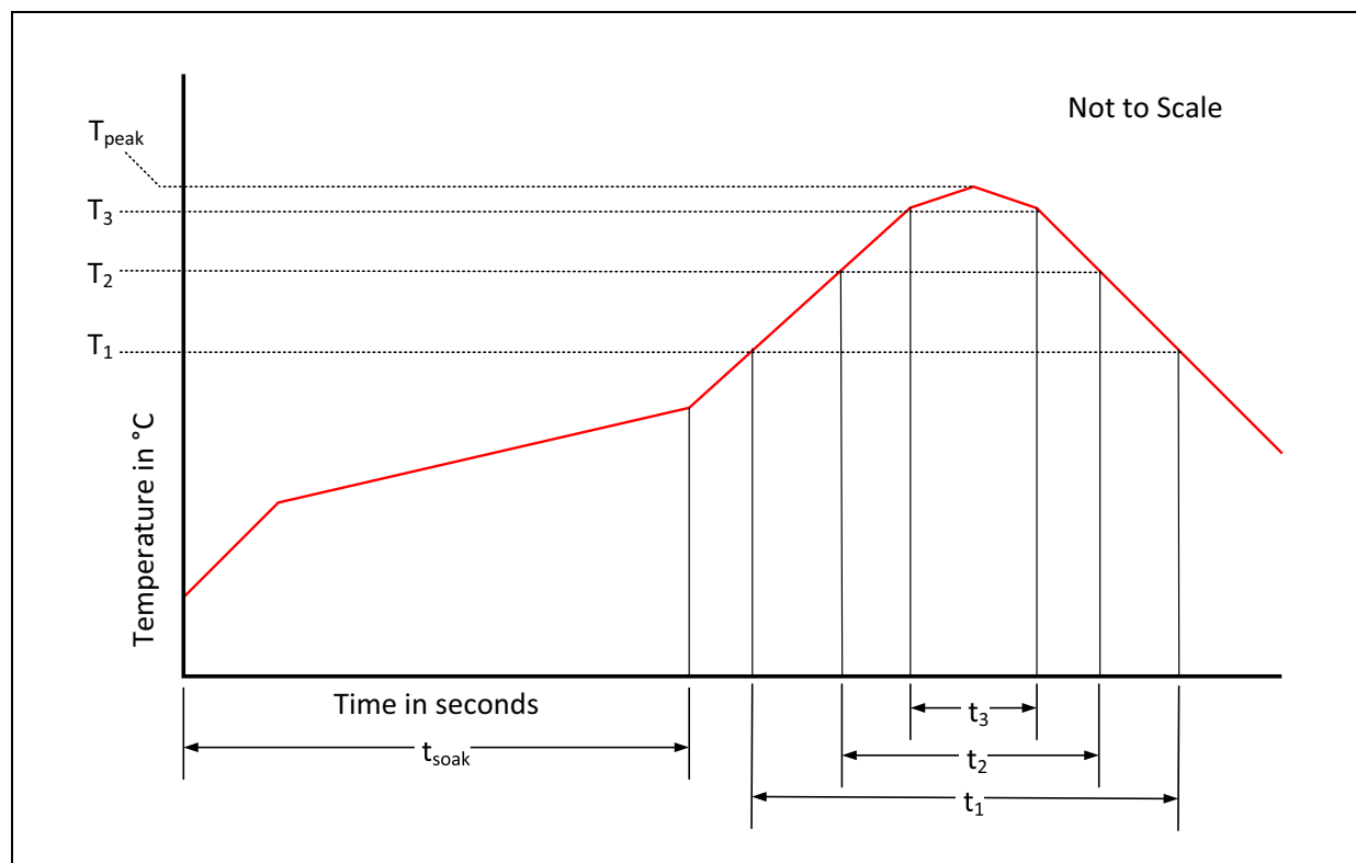
Figure 49: Solder Reflow Profile Graph
