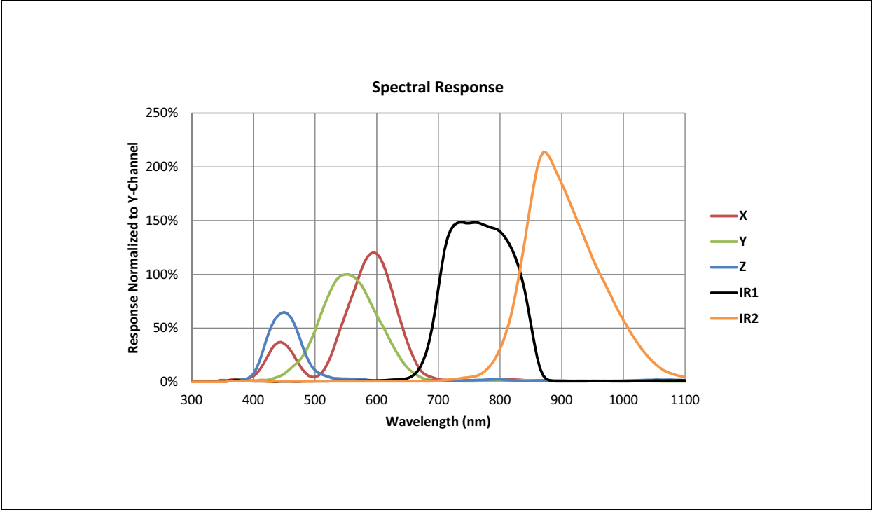
Figure 15: Spectral Response
