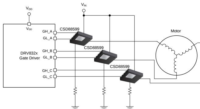
Typical Circuit
