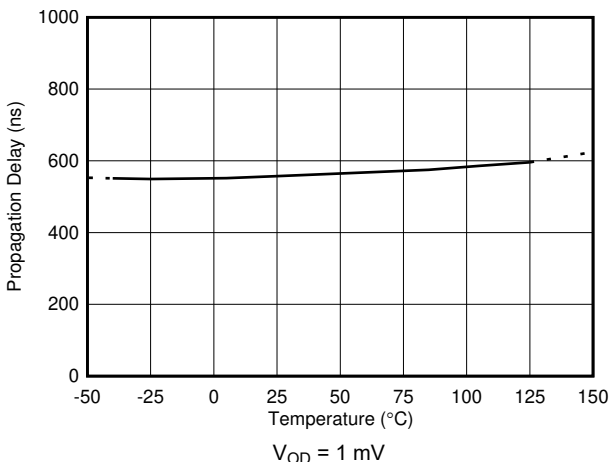
图 6-36. Comparator 1 Propagation Delay vs. Temperature
