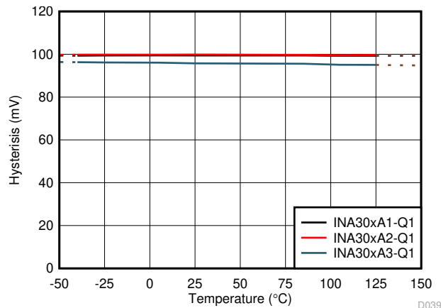
图 6-39. Comparator 1 Hysteresis vs. Temperature
