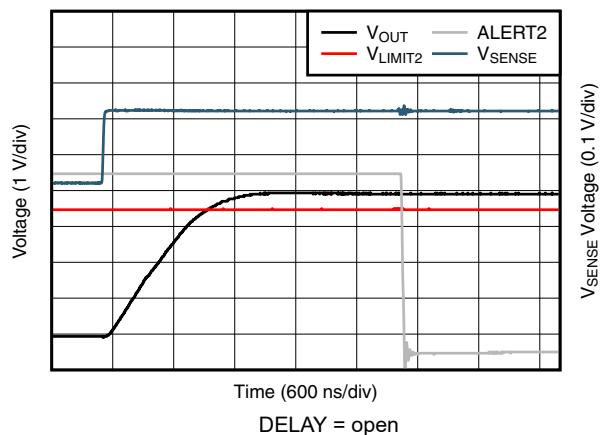
图 6-34. Comparator 2 Total Propagation Delay (INA302-Q1)
