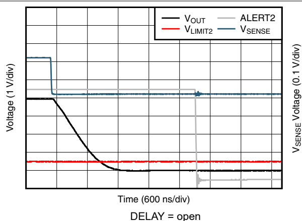
图 6-32. Comparator 2 Total Propagation Delay (INA303-Q1)
