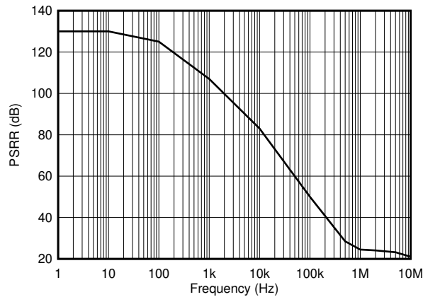
图 6-15. PSRR vs. Frequency
