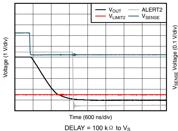
图 6-33. Comparator 2 Total Propagation Delay (INA303-Q1)
