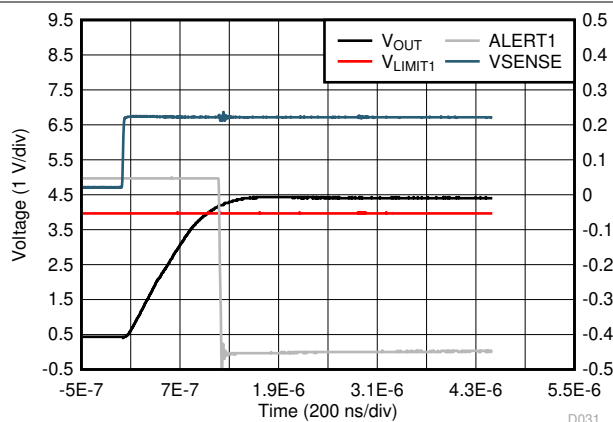
图 6-31. Comparator 1 Total Propagation Delay (INA30x-Q1)
