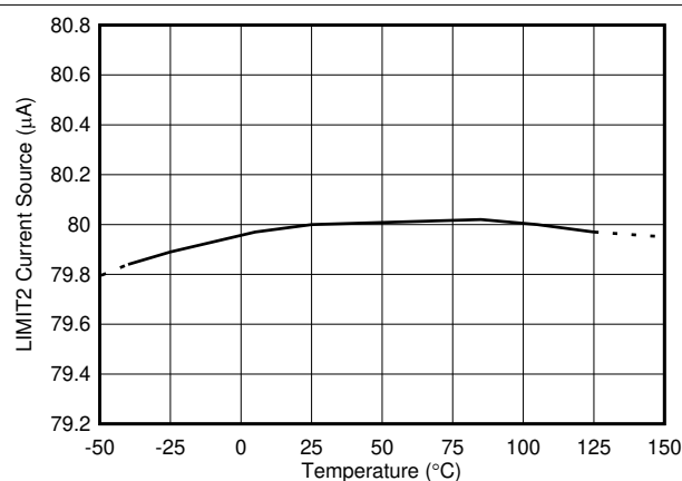
图 6-29. LIMIT2 Current Source vs. Temperature
