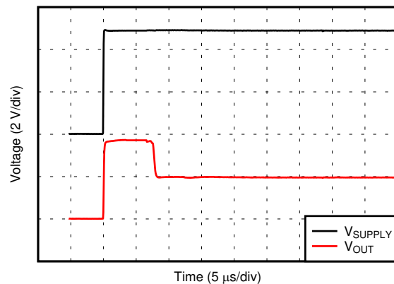
图 6-27. Start-Up Response
