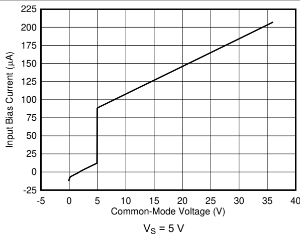
图 6-17. Input Bias Current vs. Common-Mode Voltage
