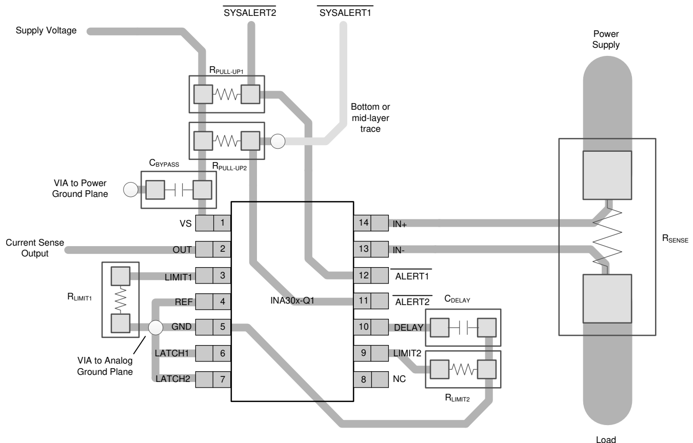
图 10-1. Recommended Layout
