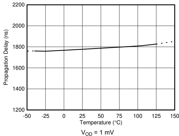
图 6-37. Comparator 2 Propagation Delay vs. Temperature
