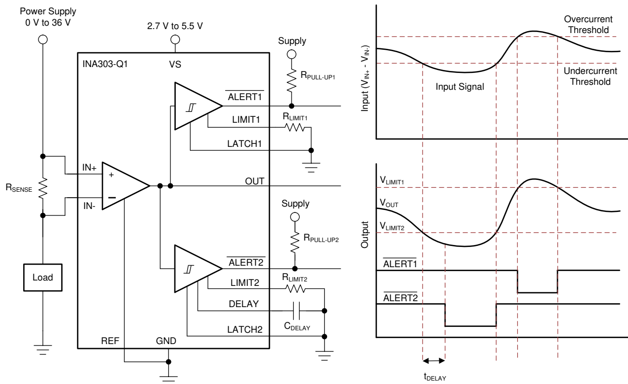
图 7-2. Out-of-Range Alert Responses for the INA303-Q1
