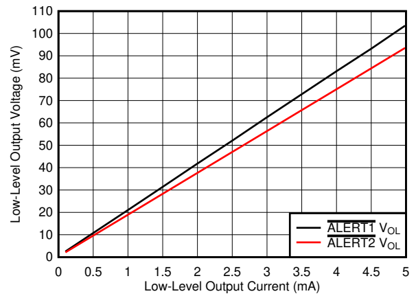
图 6-38. Comparator Alert V_{\text{OL}} vs. I_{\text{OL}}
