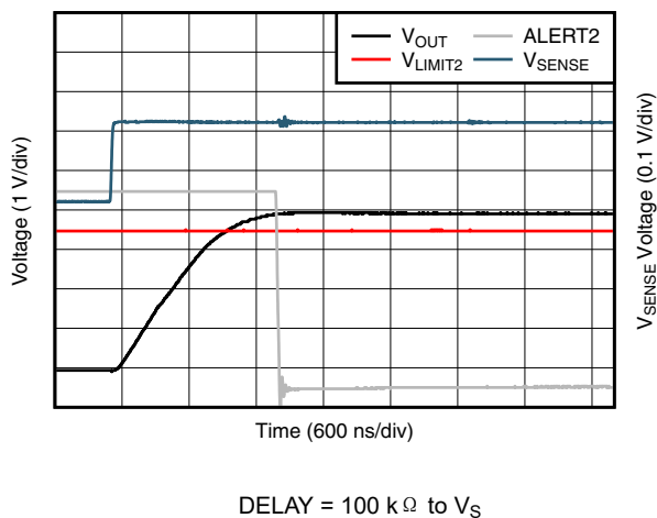
图 6-35. Comparator 2 Total Propagation Delay (INA302-Q1)
