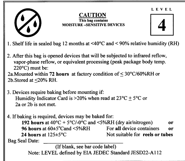
Example of JESD22-A112 Level 4 label
