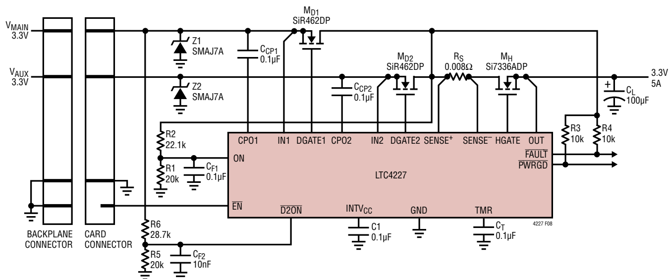
Figure 8. Plug-In Card IN1 Supply Controls the IN2 Supply Turn-On Via \overline{D2ON} Pin
