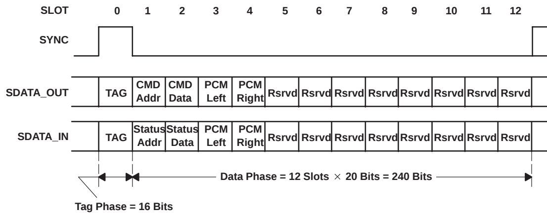
Figure 2–1. AC-Link Bidirectional Audio Frame (As Implemented)
