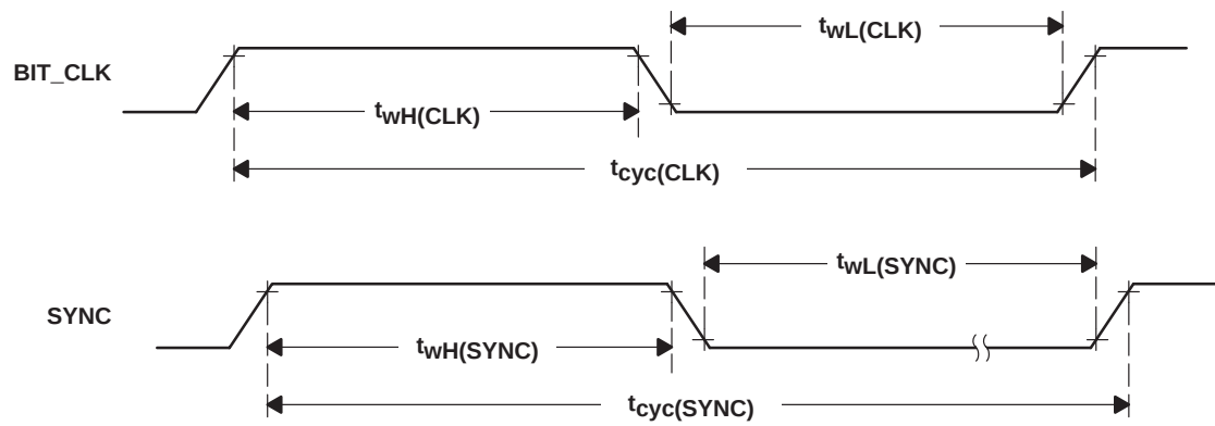
Figure 4-2. Clock Timing
